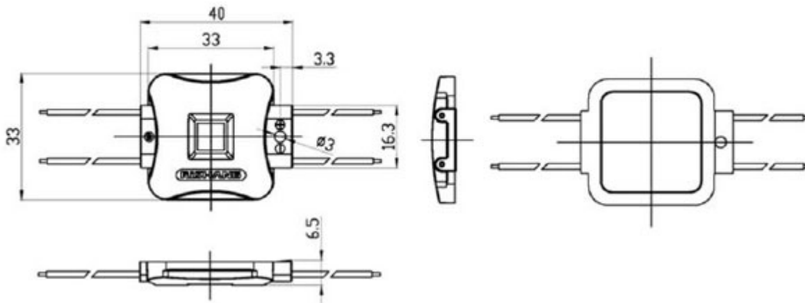
Single module dimension drawing
