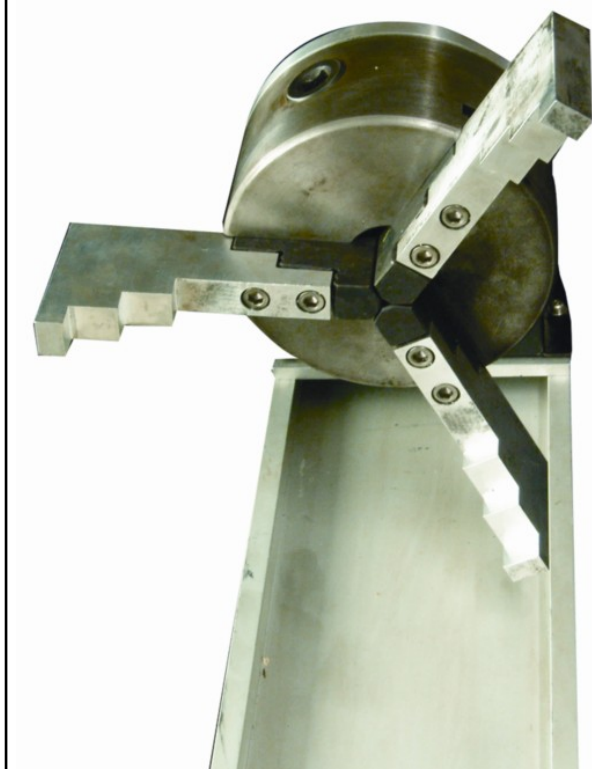
Three Claw Cylinder Fixture: Used for ?160~260mm (6"-10") column, automatic alignment center. +$926
