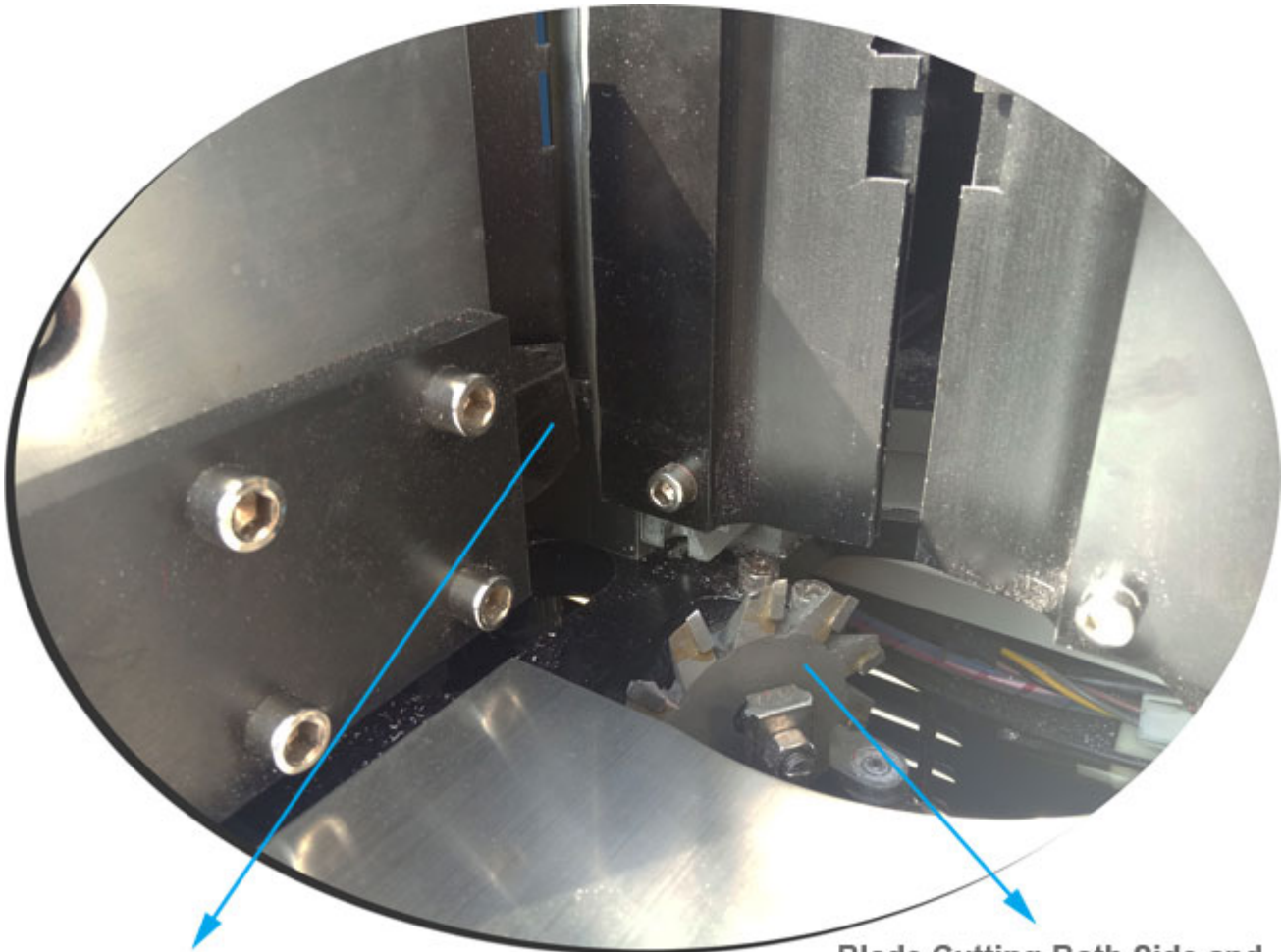
Lathe Cutting Tool-Single Side cutting
